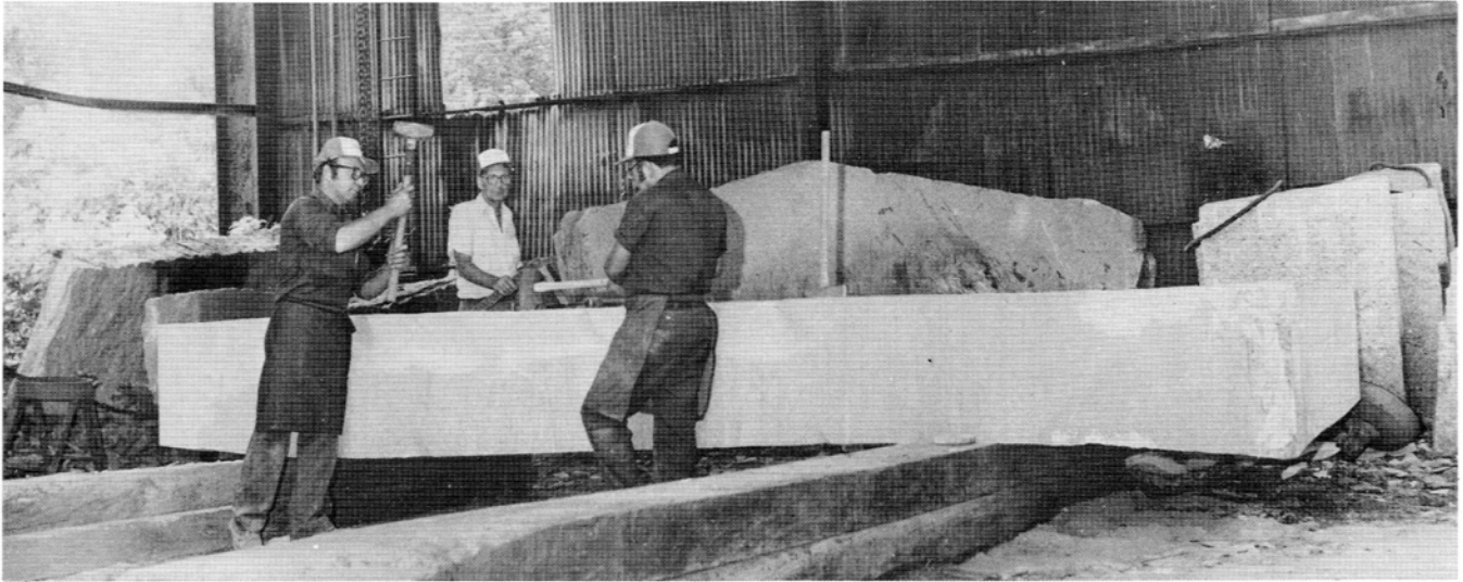
A special crew of Horace and Frankie Bradford, master stone craftsmen, under the direction of Joe B. Davis, background, a retired plant superintendent was hired to cut and pitch the granite slabs to the exact dimensions provided by "Mr. R.C. Christian." Special crews were hired because the project was so demanding that it would disrupt the regular Elberton Granite Finishing Company's production schedule.
